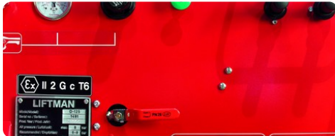
Control panel – joystick, compressed air & ATEX marking
