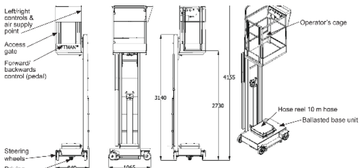
Dimensioned drawing – lift height, base and reach
