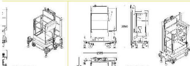
Dimensioned drawing – extended 3,140 mm / folded 2,050 mm
