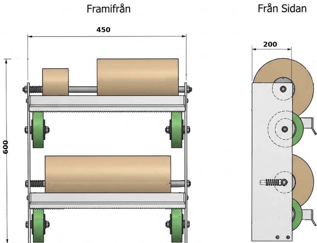
Dimensioned line drawing. All measurements in mm.
