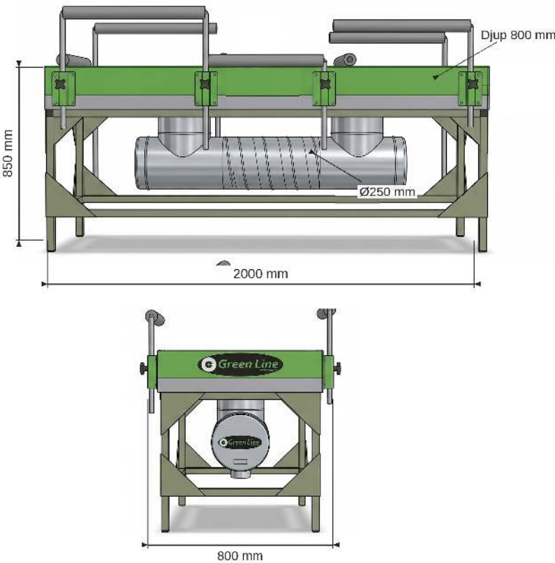
Dimensioned line drawing. All measurements in mm.
